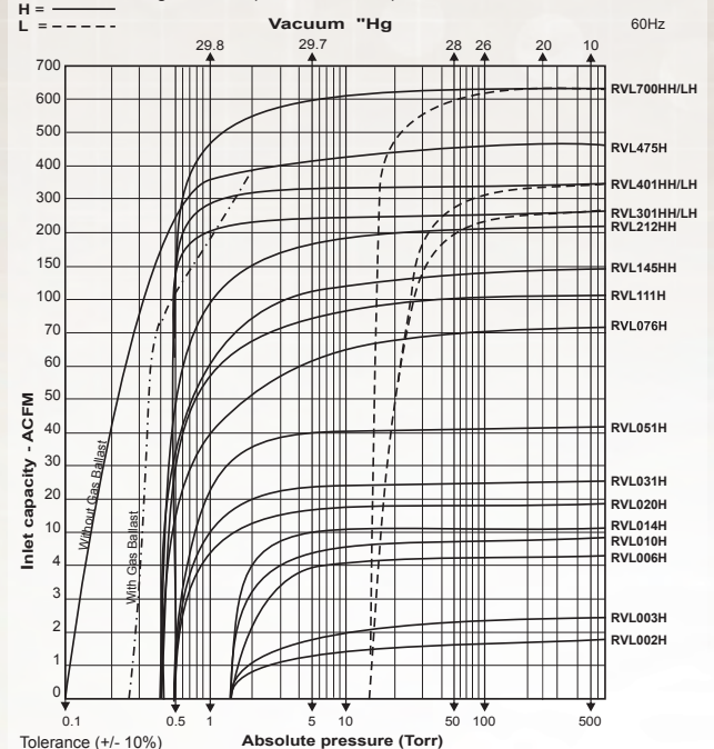
Performance curves DuraVane lubricated rotary vane pumps Based on 29.92" Hg barometric pressure, inlet temperature 70°F.
